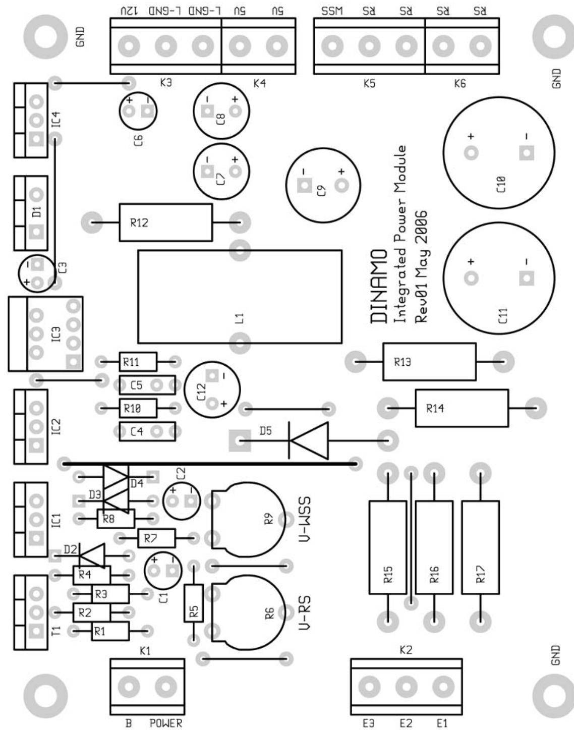
Fig 10: IPM layout
