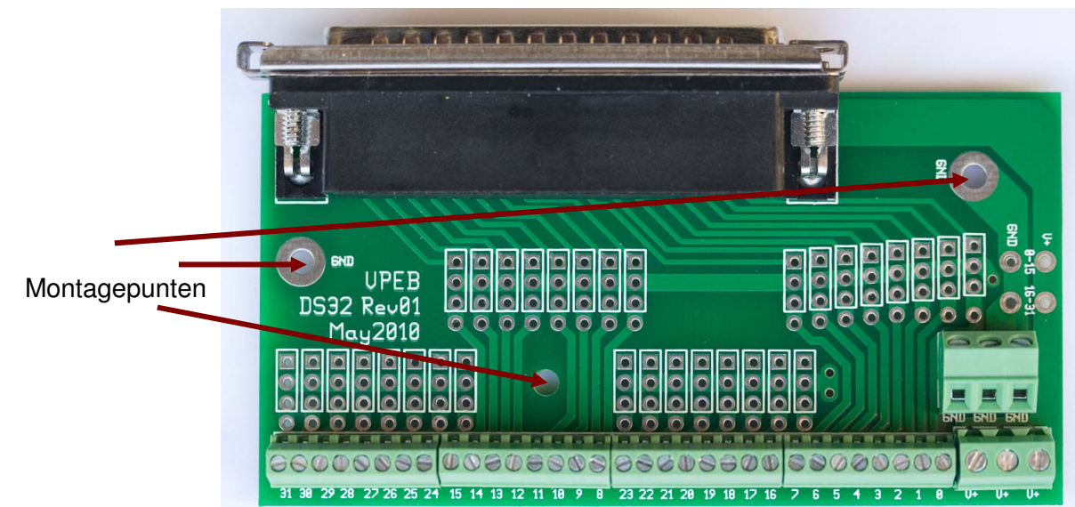
Fig 2. Layout DS32
