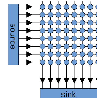
Fig 1: Multiplex Matrix
