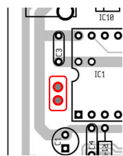
Fig 3: Pin-header
