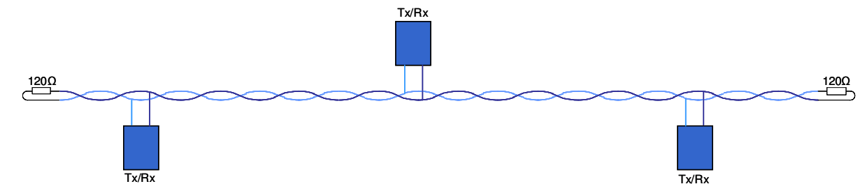
Fig 8: RS485 bus
